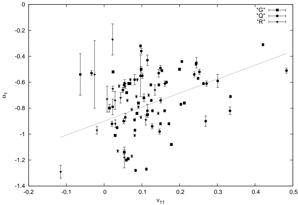
Figure 5.7: Relation between the variability index at 11 GHz v_{11} and the high-frequency spectral index \alpha_1 for galaxies (G), quasars (Q) and unidentified radio sources (R). The line is a least square fit to the data: \alpha_1 \approx 1.08(\pm 0.02) v_{11} - 0.90(\pm 0.002) .
