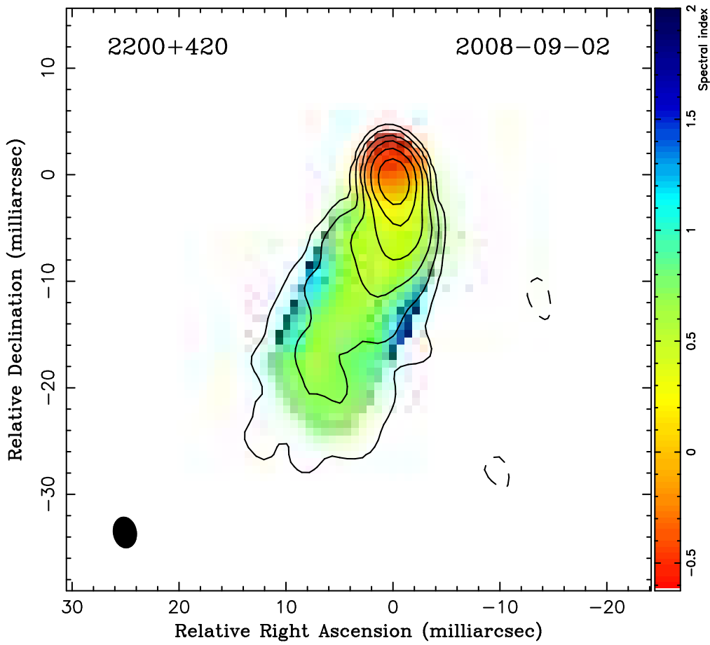
Figure 3.10: Spectral index map ( F_\nu \sim \nu^{-\alpha} , \alpha is shown in color) of BL Lacertae constructed using VLBA observations at 4.6, 5.0, 8.1 and 8.4 GHz. The overlaid contours represent total intensity at 8.4 GHz (the peak intensity is 1.75 Jy/beam, the first contour is 0.70 mJy/beam, the beam size is 1.57 \times 1.22 mas at PA = 10^\circ.4 ). The spectral index map was smoothed by a median filter with radius equal to the indicated beam size. The map shows an optically thin jet with \alpha \sim 0.7 and the self-absorbed core region ( \alpha < 0.0 ). A 2D cross-correlation technique using the optically thin part of the jet was employed to align images at different frequencies allowing reliable extraction of the spectral information. The spectral steepening towards the jet edges visible on the spectral index map occurs on the angular scale comparable to the beam size and is likely an effect of the uneven uv -coverage at different frequencies.
