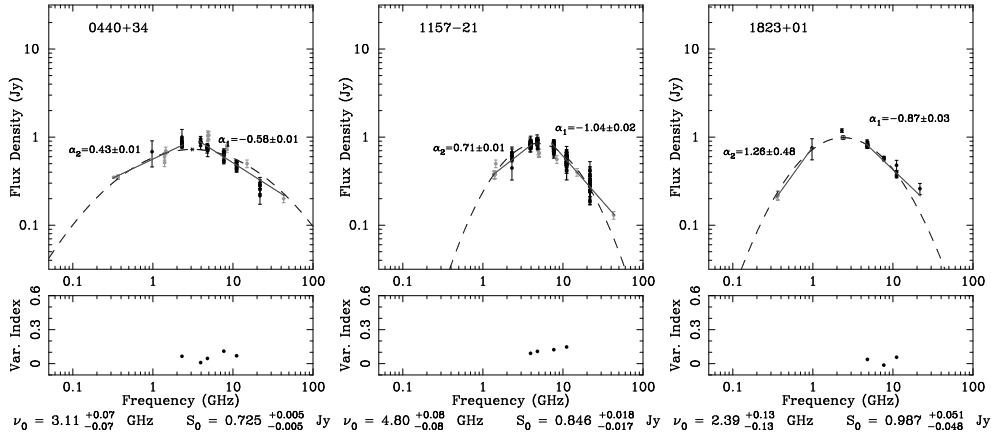
Figure 5.1: Radio spectra of 3 out of 60 newly identified GPS source candidates. Variability index as a function of frequency is presented in the panels under the spectra plots. Black points correspond to RATAN-600 data, grey points represent data collected from the literature.
