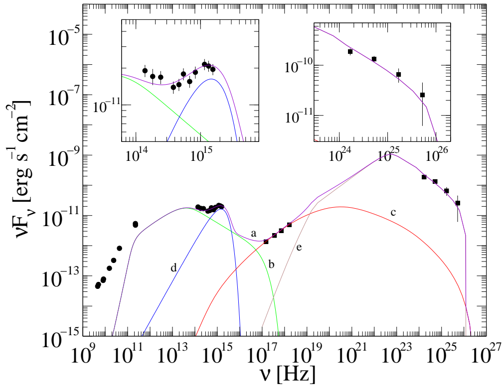
Figure 3.13: Quasi-simultaneous SED of PKS 1510–089 from Sokolovsky et al. (2010a) constructed using observations with the VLBA, Swift , Fermi /LAT, NOT, SMA and the 2.1 m telescope Guillermo Haro. The violet curve (a) represents the combined SED model: green curve (b) is the synchrotron component, red (c) is the SSC component, blue (d) is the accretion disk and brown (e) represents EC scattering of the disk radiation (see also Table 3.3).
