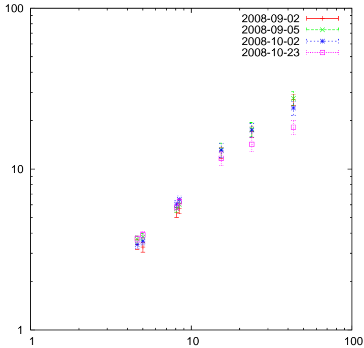
Figure 3.8: Core spectrum of 3C 454.3.
