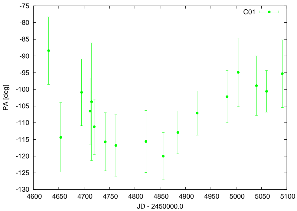
Figure 3.7: Position Angle (PA) of the component C01 with respect to the core.
