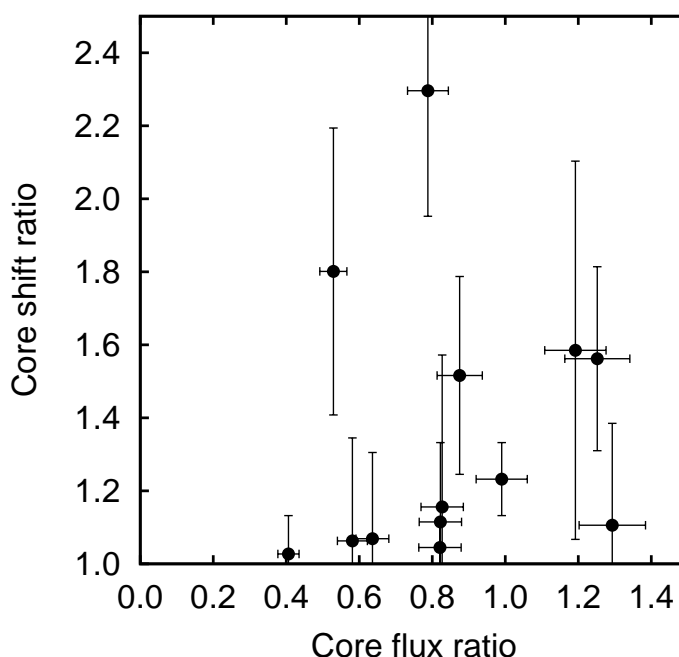
Figure 4.5: Core shift ratio versus X band core flux density ratio. The core shift ratio is defined to be greater than unity, i.e., for each pair of measurements, the larger value of the shift is in the numerator of the ratio. The one source (not shown in this plot) which exhibited a large core shift change without a major change in flux density is W Com (1219+285); it has a core shift ratio of 3.67 \pm 0.36 and core flux ratio of 1.19 \pm 0.08 .
