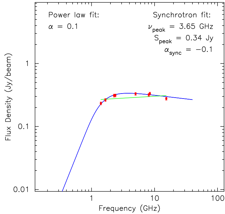
Figure 2.2: Spectrum of a single pixel (red points) in Fig. 2.1 compared to a power law (green line) and synchrotron spectrum (blue curve) fit. The synchrotron model clearly provides better fit to the data. Spatial distributions of the best-fit parameters of the synchrotron model: peak intensity S_{\text{peak}} , peak frequency \nu_{\text{peak}} and electron energy distribution index p ( p = 1 - 2\alpha , S_{\nu} \propto \nu^{\alpha} ) are presented on Fig 2.1b, 2.1c and 2.1d respectively.
