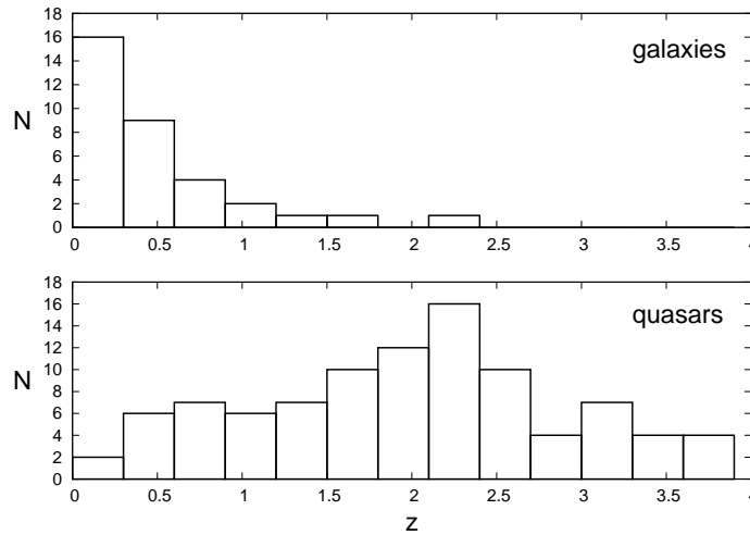
Figure 5.6: Redshift distribution of GPS galaxies and GPS quasars from the sample.
