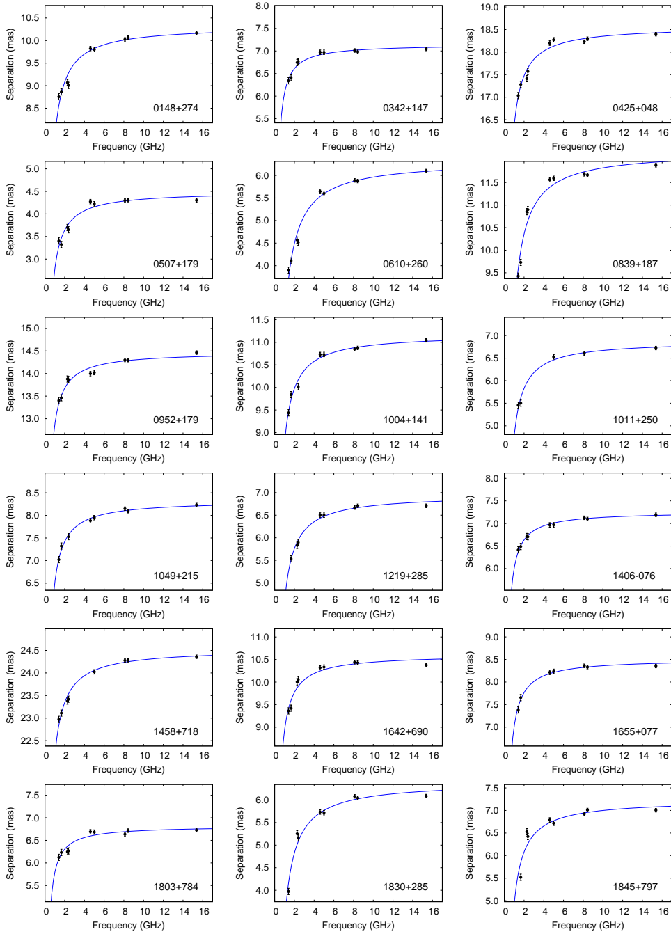
Figure 4.2: Separation of the core from a reference optically-thin jet component as a function of frequency. The curve represents the best-fit function r_c(\nu) = a + b\nu^{-1/k} , the coefficient k = 1 was fixed during the fitting. The best-fit parameters are presented in Table 4.4.
