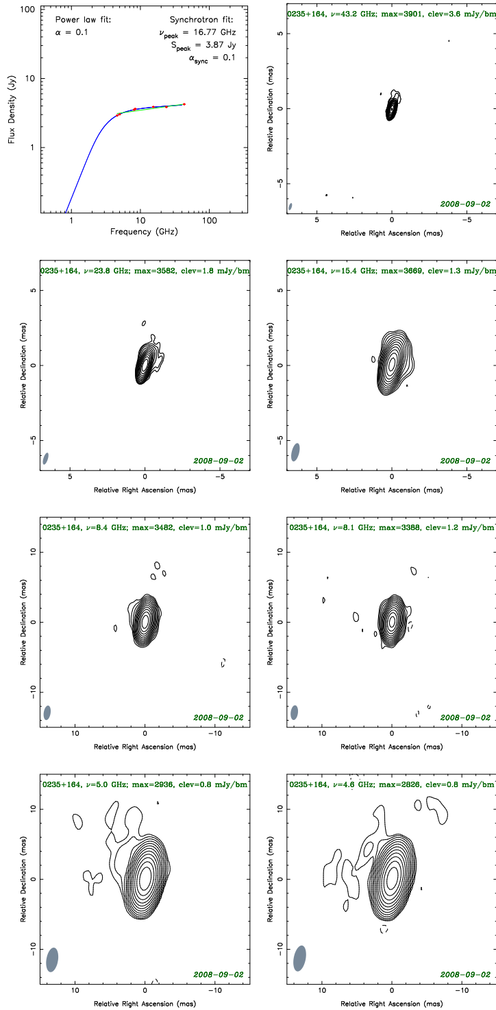
Figure 2.3: Spectrum of the core and naturally weighted CLEAN images of the \gamma -ray bright blazars observed with the VLBA between 4.6 and 43.2 GHz. The lowest contour value ‘clev’ is chosen at four times the rms noise, the peak brightness is given by ‘max’. The contour levels increase by factors of two. The dashed contours indicate negative brightness. The half power beam width is shown in the bottom left corner of the images in grey. An epoch of observation is shown in the bottom right corner.
