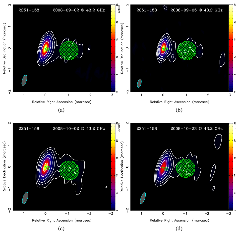
Figure 3.1: Total intensity VLBA images of 3C 454.3 at 43.2 GHz at four epochs covered by our multifrequency observations. Image details: 3.1a – peak 24.6 Jy/beam, first contour 0.030 Jy/beam; 3.1b – peak 23.4 Jy/beam, first contour 0.030 Jy/beam; 3.1c – peak 21.7 Jy/beam, first contour 0.015 Jy/beam; 3.1d – peak 15.6 Jy/beam, first contour 0.020 Jy/beam. Contours are a factor of 4 apart in all cases. The beam is plotted in the lower left corner of each image. Green circles represent Gaussian components used to model the 43.2 GHz brightness distribution of the source.
