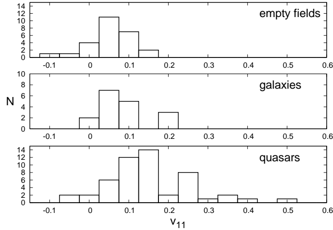
Figure 5.5: Distribution of the observed variability index v_{11} at 11 GHz for GPS quasars, galaxies and unidentified radio sources (empty fields) in our sample.
