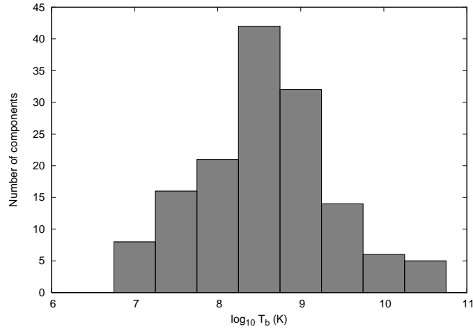
Figure 5.16: Brightness temperature distribution (measured at 8 GHz) for bright CSO components.
