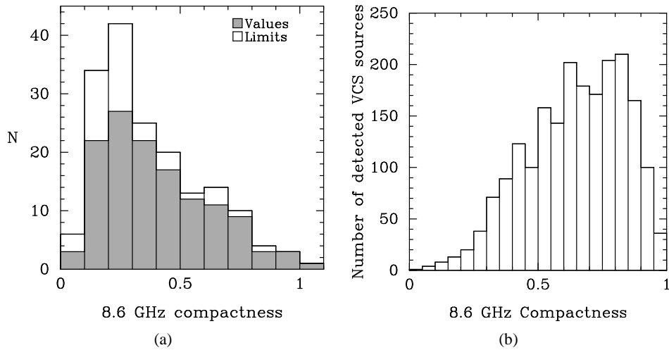
Figure 5.11: “Compactness index” for sources from the RATAN–600 GPS sample (a) and from the complete sample of flat spectrum sources (b).
