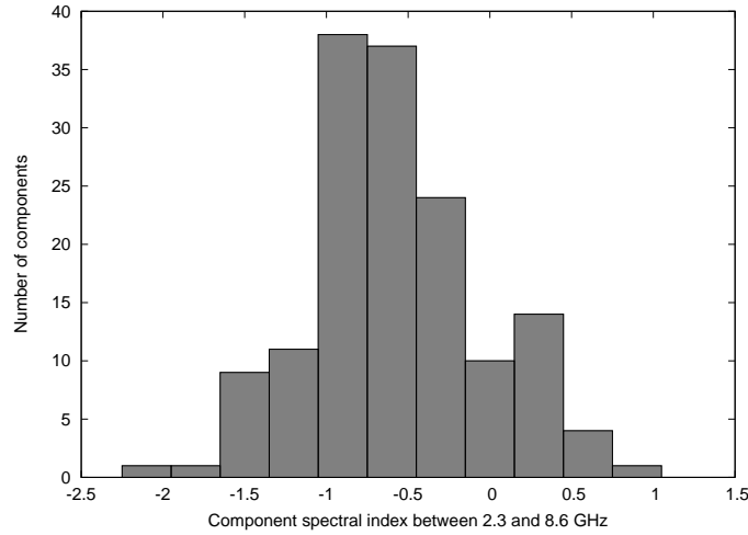
Figure 5.14: Spectral index, \alpha , distribution (2 – 8 GHz) for bright CSO components ( F_\nu \propto \nu^\alpha ).
