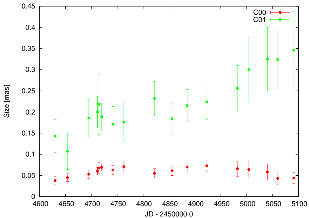
Figure 3.5: Size of the first jet component (C01) and the core (C00) as a function of time.
