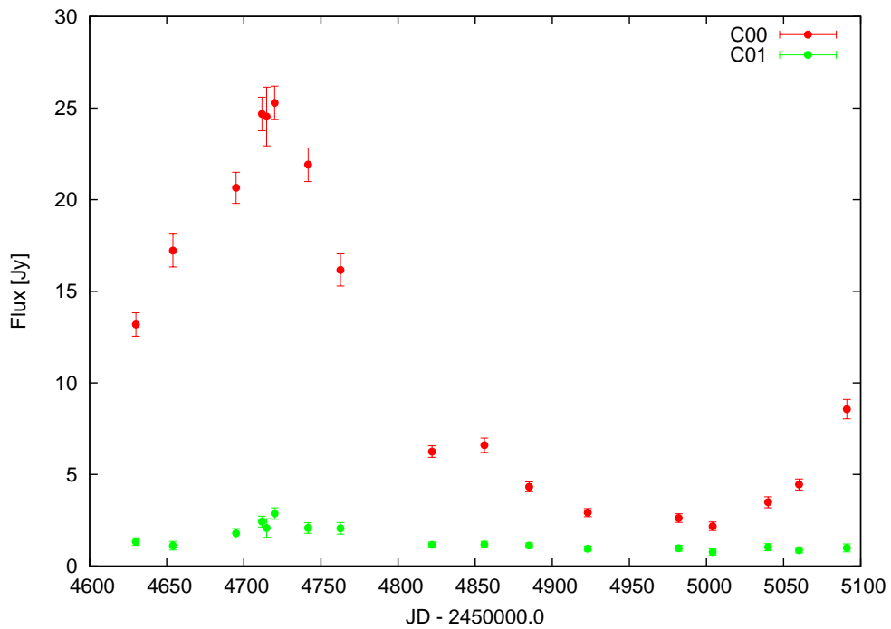
Figure 3.4: Lightcurve of the 43 GHz core of 3C 454.3 (marked “C00”) and the first jet component “C01” about 0.15 mas away from the core.
