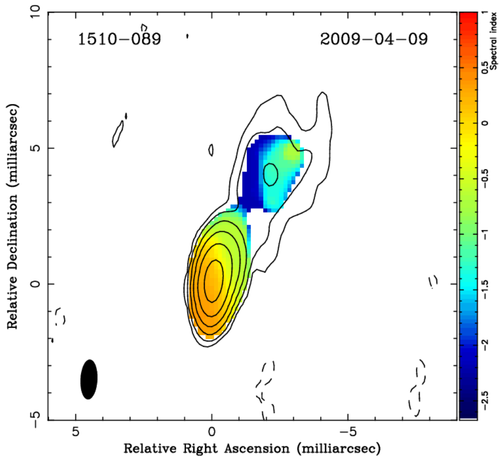
Figure 3.12: Spectral index \alpha ( F(\nu) \propto \nu^\alpha ) map between 15.4 and 23.8 GHz (shown in color) of PKS 1510-089 as observed by the VLBA on 2009 April 9. The overlaid contours represent total intensity at 15.4 GHz (see Figure 3.11 for details). The spectral index map was smoothed by a median filter with a 0.6 mas radius.
