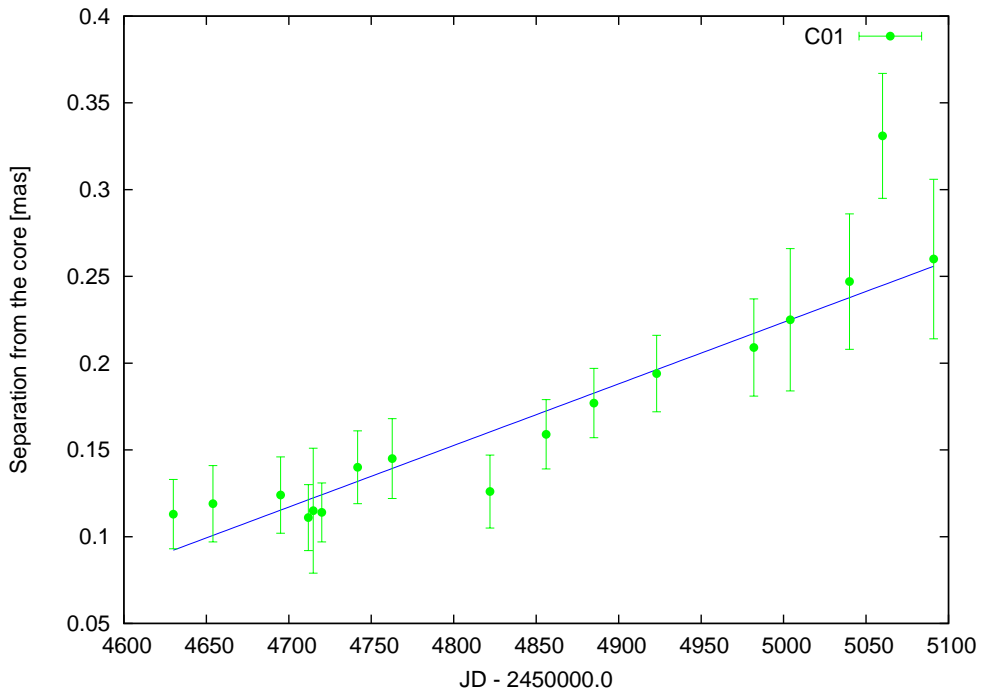
Figure 3.6: Separation of the component “C01” from the core (“C00”) of 3C 454.3 as a function of time. The blue line represents the least square fit to the data.
