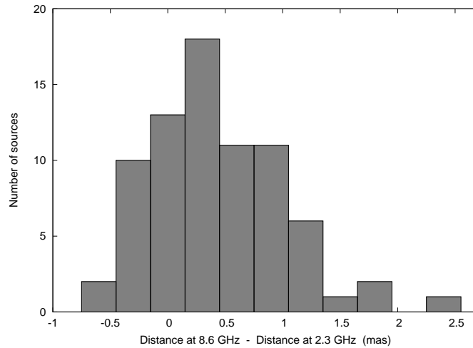
Figure 5.17: Difference in distances between two dominating source components measured at 2 and 8 GHz. The median value of the distribution is 0.39 which is significantly (99.9997 % probability according to the sign test) greater than zero.
