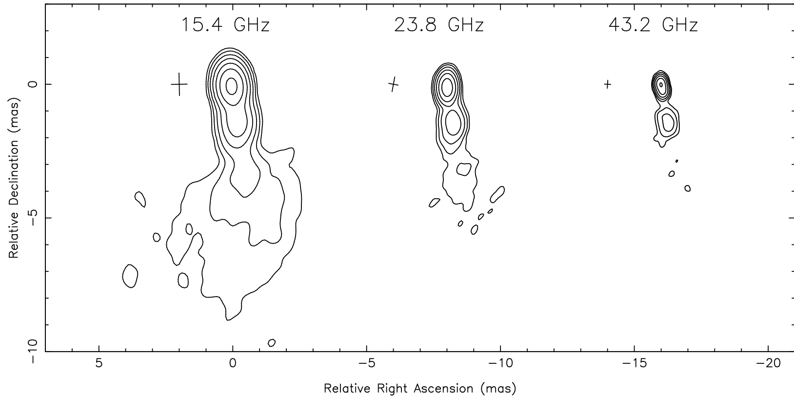
Figure 3.9: Inner jet of BL Lacertae as observed by the VLBA on September 02, 2008. Images at different frequencies are shifted by 8 mas in relative Right Ascension. For the 15.4, 23.8 and 43.2 GHz image map peaks are 1.69, 1.52, 1.32 Jy/beam, first contours are 1.70, 3.00, 5.00 mJy/beam respectively. The contour levels are increased by a factor of 3. Beam size (natural weighting) for each frequency is indicated by the cross to the left of the corresponding image.
