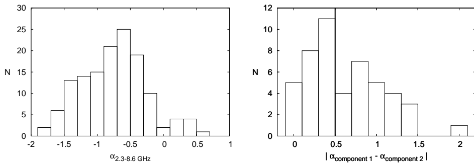
(a) Spectral indices of individual components (b) Difference between spectral indices of components
