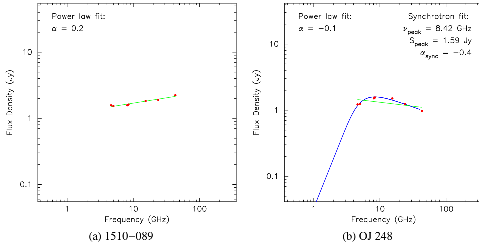
Figure 2.4: VLBA spectra of core regions of 1510–089 (a) and OJ 248 (b). The former spectrum is flat while the latter one shows a prominent synchrotron self-absorption peak. The green line is a power law fit. The blue curve is a homogeneous synchrotron source model.
