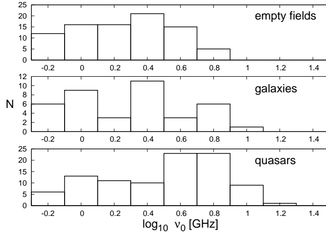
Figure 5.3: Peak frequency distribution for GPS quasars, galaxies and unidentified radio sources (empty fields).
