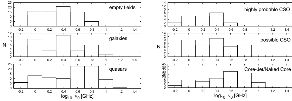
Figure 5.10: Observed peak frequency distribution for GPS sources with different optical identification and parsec-scale radio structure.
