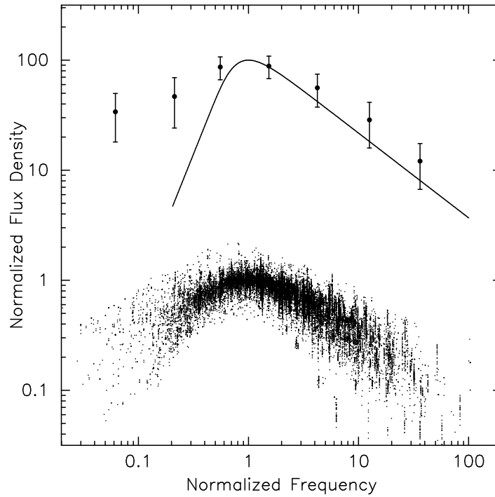
Figure 5.2: Combined spectra of all selected 226 GPS candidates normalized by peak flux density and peak frequency values. Filled circles represent the observed spectra binned and shifted along the vertical axis. The solid line is a normalized and shifted theoretical spectrum of a homogeneous synchrotron emitting cloud with self-absorption and power index \gamma = 2.54 of the electron energy distribution.
