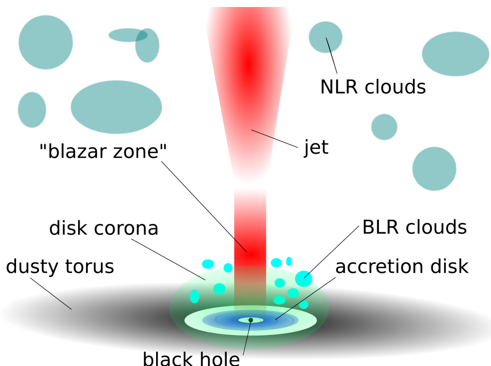
Figure 1.1: Scheme of a radio-loud AGN. Note that relative sizes are not to scale and shapes of many structures (like the Broad Line Region – BLR and Narrow Line Region – NLR) are very uncertain. The “blazar zone” is likely a small section of the inner jet, presumably located inside or just outside the BLR. The “blazar zone” is responsible for relativistically-beamed, highly variable emission at NIR and optical bands and at high energies.
