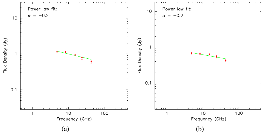
Figure 3.14: The VLBA spectrum of Mrk 501: 3.14a — integrated parsec-scale spectrum, 3.14b — core spectrum.
