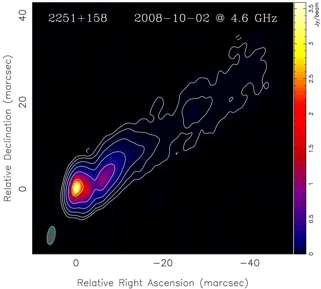
Figure 3.2: Total intensity VLBA image at 4.6 GHz. The first contour is 0.002 Jy/beam, factor = 4. The beam is shown in the lower left corner of the image.
