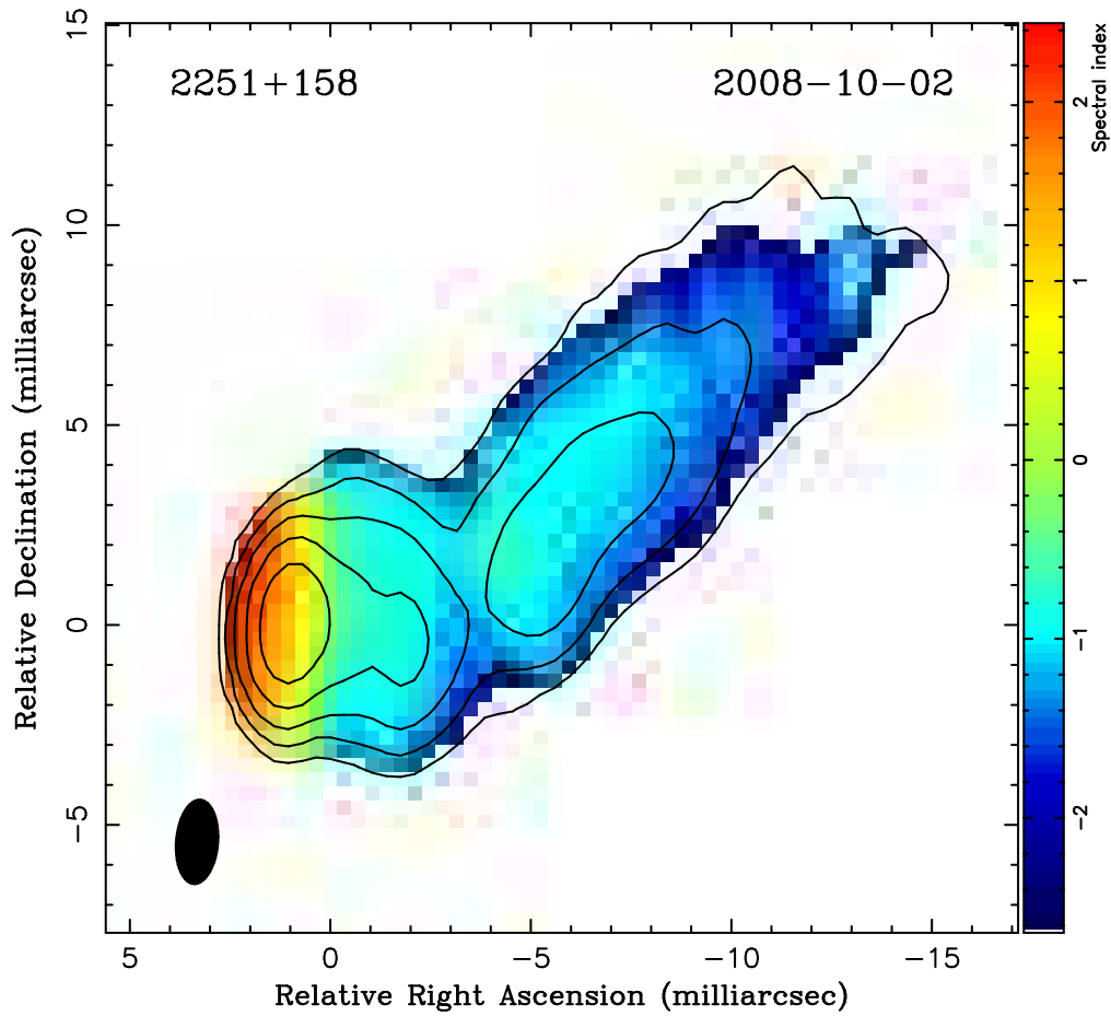
Figure 3.3: Spectral index map constructed by fitting a power law to observations at three frequencies: 8.1, 8.4 and 15.4 GHz. Contours represent total intensity at 8.4 GHz. Contour map peak = 6.442 Jy/beam, first contour 0.1% of the peak. Beam FWHM = 2.12 \times 1.05 mas at PA = -4^{\circ}.64 .
