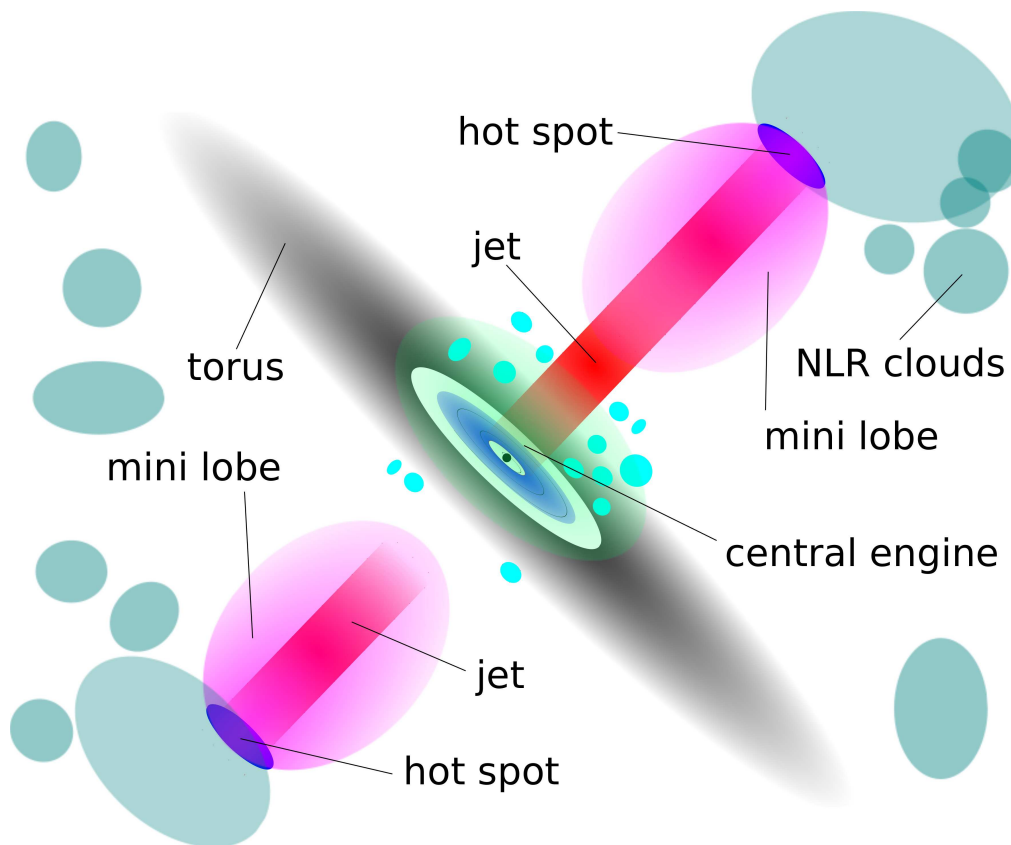
Figure 1.4: Scheme of a Compact Symmetric Object (CSO) – a miniature radio source contained entirely within the Narrow Line Region (NLR) of its host galaxy.
