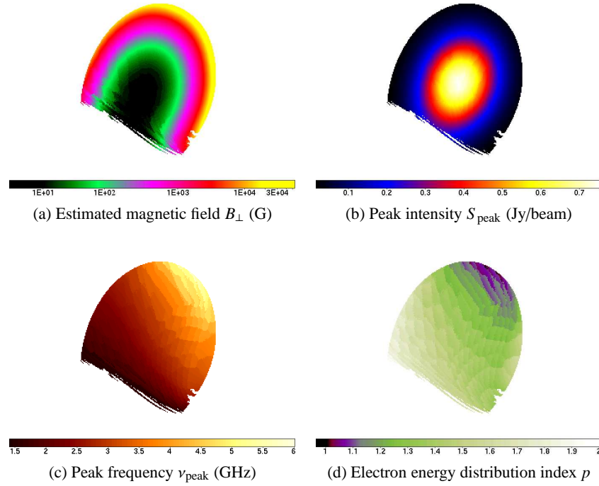
Figure 2.1: Maps of the best-fit synchrotron spectrum (Fig. 2.2) parameters and the estimated magnetic field strength derived from nine images (1.4–15.4 GHz range) of the source 1458+718 convolved with the same Gaussian beam. From this example it is clear why convolution with a Gaussian beam makes VLBI images unsuitable for magnetic field estimation. The convolved images have large areas of artificial low flux surrounding each area where the actual flux is detected (see the distribution of the peak intensity at Fig. 2.1b). These artificial low-flux areas (where there should be no flux at all) result in very high estimated values of B_{\perp} (Fig. 2.1a) around each spot with actual detected flux (and, therefore, a valid estimation of B_{\perp} ). The peak frequency (Fig 2.1c) and power index of the electron energy distribution (Fig 2.1d) do not change much across the area and the effect of their changes is negligible compared to the effect of convolution. We note that only pixels where spectral turnover was detected (i.e. the spectrum in such pixel significantly deviates from a power law) are shown on the images.
