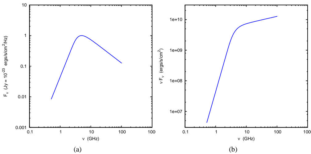
Figure 1.5: Theoretical spectrum of a uniform synchrotron source (Section 1.3.1) plotted in spectral ( F_\nu , 1.5a) and SED ( \nu F_\nu , 1.5b) coordinates.
