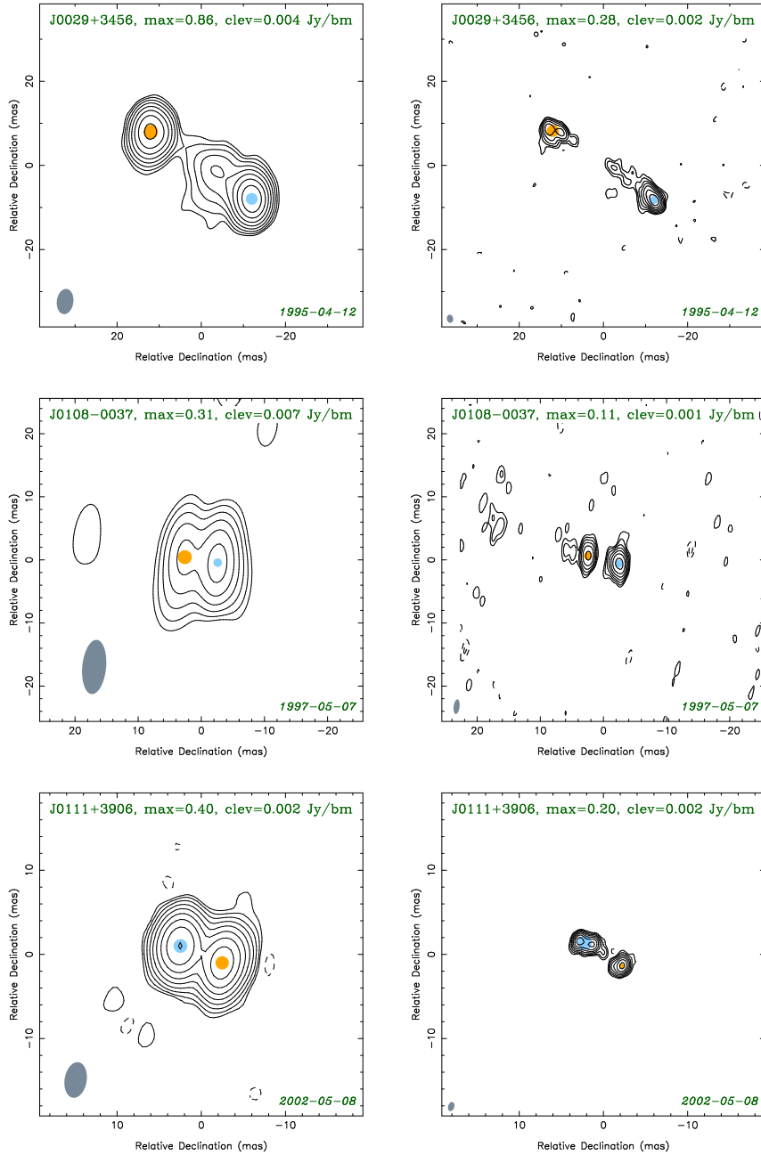
Figure 5.13: Dual-frequency simultaneous 2 and 8 GHz naturally weighted CLEAN images. The lowest contour value ‘clev’ is chosen at four times the rms level, the peak brightness is given by ‘max’ (Jy/beam). The contour levels increase by factors of two. The dashed contours indicate negative flux. The beam is shown in the bottom left corner of the images. An epoch of observation is shown in the bottom right corner. Light blue and orange spots indicate Gaussian model components 1 and 2 respectively.
