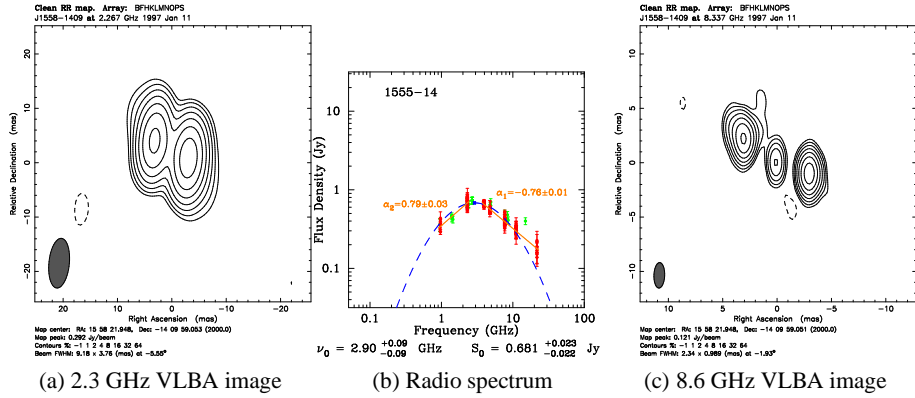
Figure 5.9: PKS 1555–140 – new GPS galaxy with CSO morphology at z = 0.097 . Red points on the panel (b) denote RATAN–600 observations, green points represent literature data.
