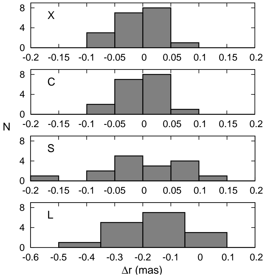
Figure 4.3: Distribution of the observed difference in distance between the core and reference component measured at two sub-bands of X , C , S and L band.
