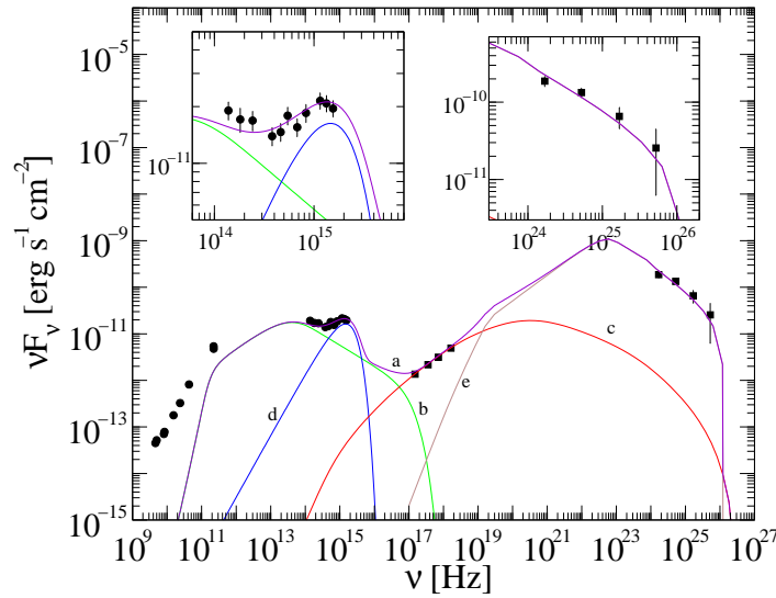
Figure 1.2: The observed Spectral Energy Distribution (SED) of a quasar-type blazar compared to a model. See Fig. 3.13 and Section 3.3 for a detailed discussion.
