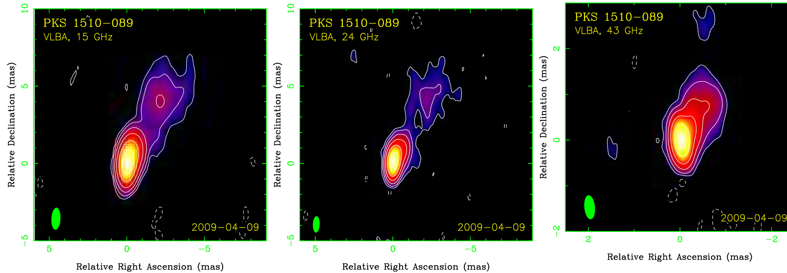
Figure 3.11: Stokes I CLEAN images of PKS 1510-089 observed by VLBA on 2009 April 9, at 15, 24, and 43 GHz. The lowest contour and peak intensity are 0.7 mJy/beam and 1.47 Jy/beam (15 GHz), 0.7 mJy/beam and 1.56 Jy/beam (24 GHz), 2 mJy/beam and 1.85 Jy/beam (43 GHz). Contours are plotted with a step \times 4 . Natural weighting of visibility data is used, HPBW beam size is shown in the lower left corner. Angular size of 1 mas corresponds to 5 pc.
