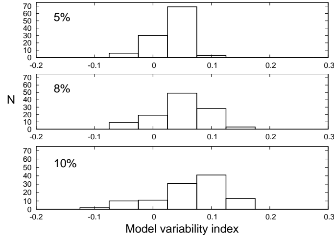
Figure 5.4: Distribution of variability index \nu for the model non-variable sources measured with the relative accuracy of 5, 8 and 10% respectively.
