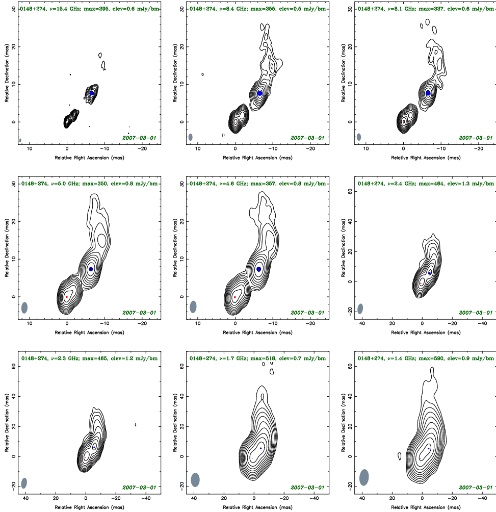
Figure 4.1: Naturally weighted CLEAN images of the observed sources between 1.4 and 15 GHz. The lowest contour value ‘clev’ is chosen at four times the rms noise, the peak brightness is given by ‘max’. The contour levels increase by factors of two. The dashed contours indicate negative brightness. The beam’s full width at half maximum (FWHM) is shown in the bottom left corner of the images in grey. An epoch of observation is shown in the bottom right corner. Red and blue spots indicate the positions and sizes (FWHM) of Gaussian model components for the core and the jet features respectively.
