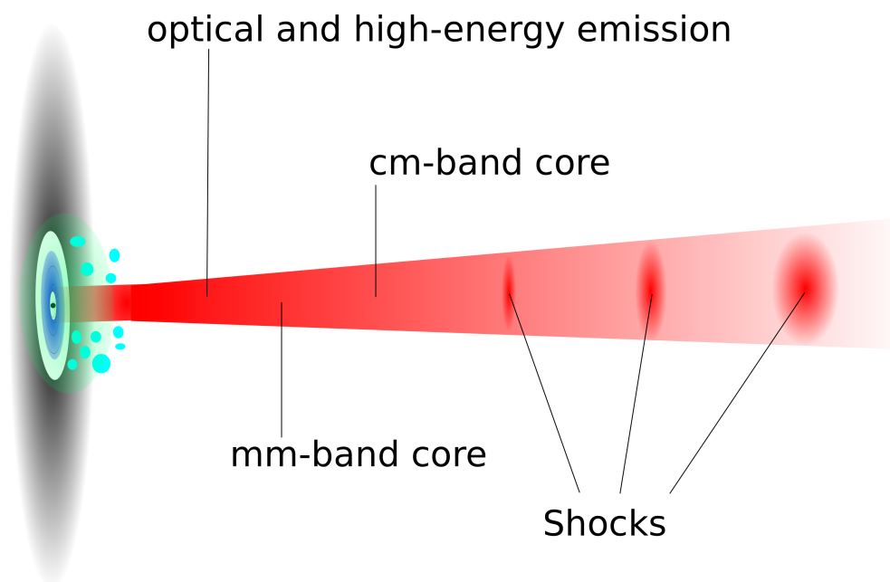
Figure 1.3: Scheme of a blazar jet. Note that mm-band core is located upstream (closer to central engine) than cm-band core due to the “core shift” effect. At any given frequency, sections of the jet upstream from the core corresponding to this frequency are hidden from sight by opacity. The “blazar zone”, site of the NIR, optical and high-energy emission, is located upstream from the mm-band core. Shocks traveling the jet could potentially also be responsible for a fraction of high-energy emission.
